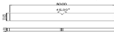
Impact test specimen; ASTM D256 / ISO 179, GB/T 1043
